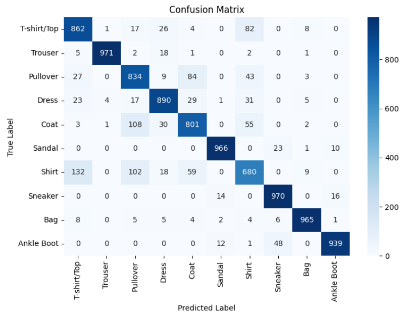
Figure 7: Confusion Matrix
